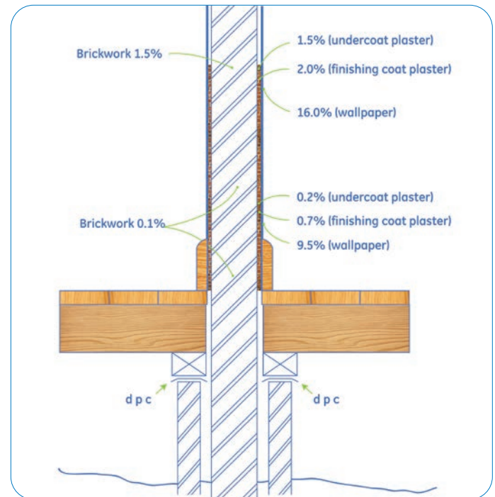
Concentration of salts in a party wall in which rising damp has persisted for 80 years. The figures show the percentage by weight of chloride plus nitrate. The shaded area is heavily contaminated. (Redrawn from Building Research Establishment Digest 245. revised 1987)
